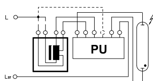
Ballasts with two tapping points and two voltage tapping points (L ST = 0 V or L ST > 0 V)
