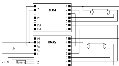
2-lamp operation – Dimming with electronic ballast ELXd
