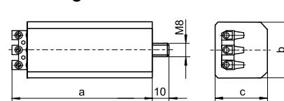
PC casing
