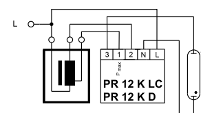
Electronic power reduction without control phase
